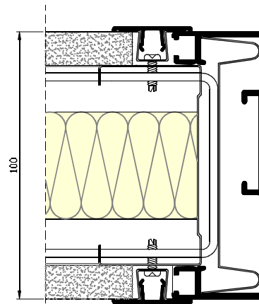
C | detail
